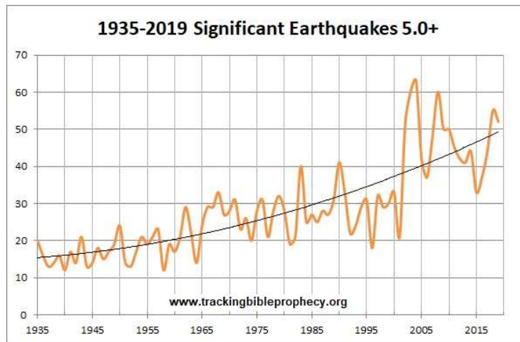
Figure 14: Earthquake Trends
